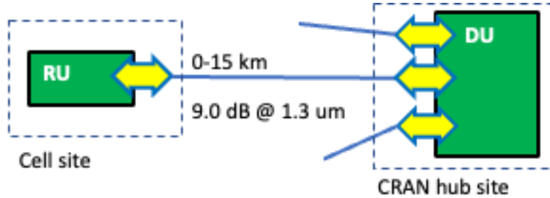
Figure 15: 15 km RU-DU direct parallel fibers Blueprint. Note 8.3.2
