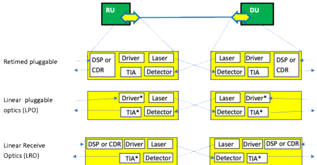
Figure 39: Illustration of retimed, linear (LPO) and linear receive (LRO) optical pluggables in an LLS example with RU and DU. * Indicates that the laser Driver and TIA (transimpedance amplifier) in the linear implementations may be enhanced with channel equalization capabilities.
