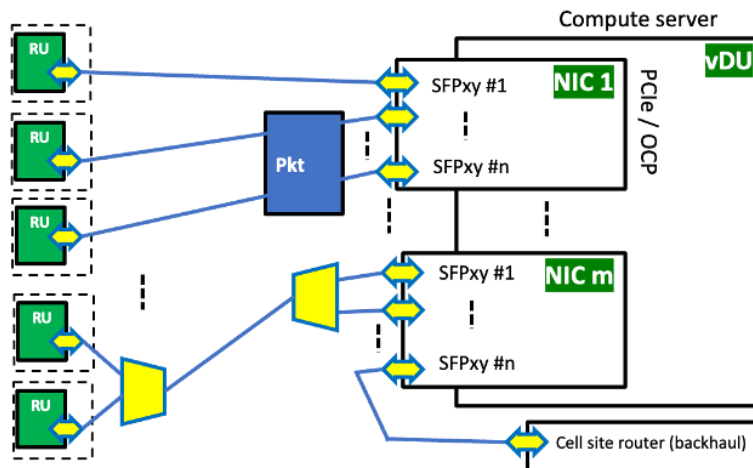
Figure 35: Cloud RAN optical solution. Several connectivity solutions between vDU and RU are show (from top to bottom) parallel dual or bidi gray fibers, packet aggregation and DWDM aggregation.
