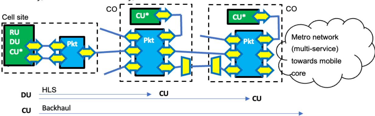
Figure 23: Backhaul and HLS for DRAN and virtual RAN. CU* indicates possible locations for the CU, at the cell site, or at the closest CO. The latter constitutes the VRAN case. The pluggables at the CO sites may be C-temp as indicated by dashed borders for the intraoffice ones.
