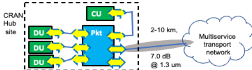
Figure 30: 10 km CRAN backhaul Blueprint (direct P2P, no WDM). The link specified has a gray background. In cases where the CU is located at another location, HLS is illustrated. The pluggables at the CRAN hub site may be C-temp as indicated by dashed borders for the intraoffice ones.
