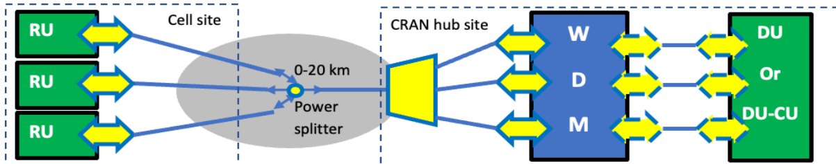
Figure 38: LLS using semi-active DWDM wavelength multiplexed links over a power splitter ODN (WS-WDM-PON).
