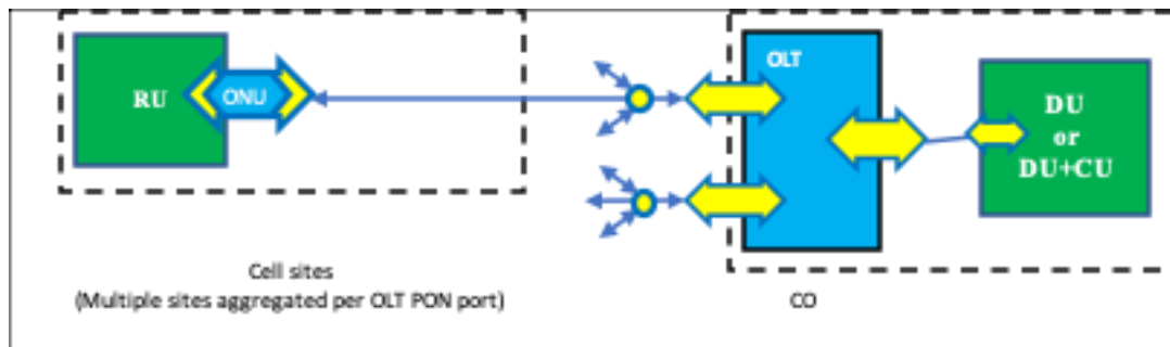
Figure 37: LLS using TDM-PON with a pluggable ONU module.
