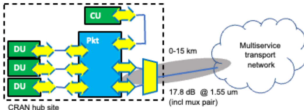
Figure 31: 15 km CRAN backhaul, DWDM passive wavelength multiplexed Blueprint. In cases where the CU is located at another location, HLS is illustrated.
