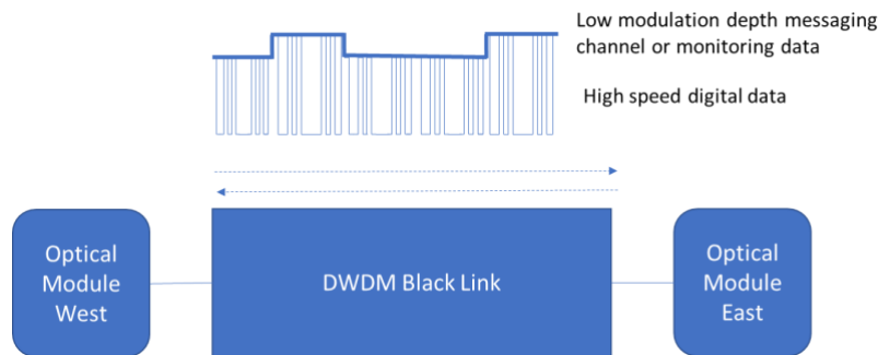
Figure ANB.1: Optical modules exchanging messaging channel and monitoring data over a DWDM black link 11 (as an example).
