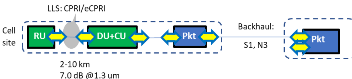
Figure 13: 10 km RU-DU direct parallel fibers Blueprint.
