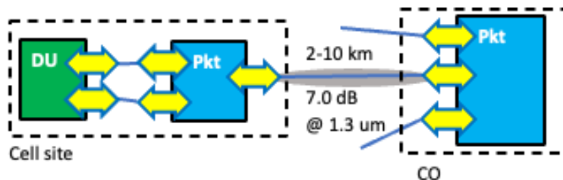
Figure 25: 10 km DRAN backhaul with direct parallel fiber, dual or BiDi Blueprint. The link specified has a gray background. In cases where the cell site DU is collocated with the CU, backhaul is illustrated. If the CU is located at another location, HLS is illustrated.
