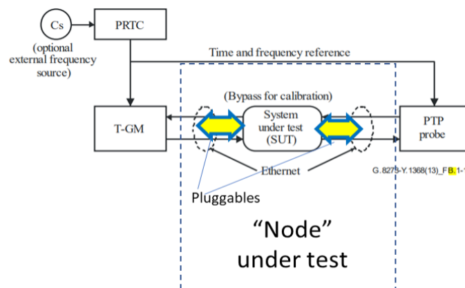
Figure APB.6: Figure B.1.1 from G.8273.2 Annex B.
