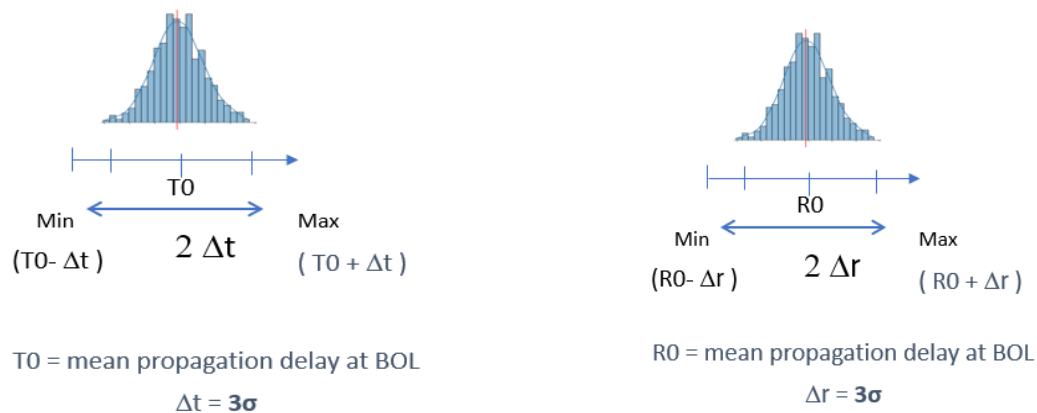
Figure APB.11: histogram measurements
