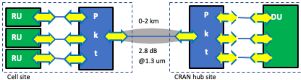
Figure 20 : 2 km RU-DU, packet multiplexing, P2P or P2MP Blueprint. The link specified has a gray background. There may be additional intermediate Pkt nodes between the depicted Pkt node and DU, for example on case of cloud RAN deployments at the hub site. The intraoffice pluggables at the hub site may be C-temp as indicated by dashed borders.
