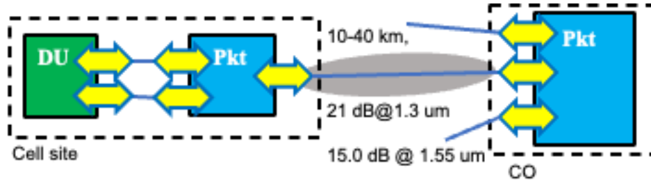
Figure 26: 40 km DRAN backhaul direct parallel fiber, dual or BiDi Blueprint. The link specified has a gray background. In cases where the cell site DU is collocated with the CU, backhaul is illustrated. If the CU is located at another location, HLS is illustrated.
