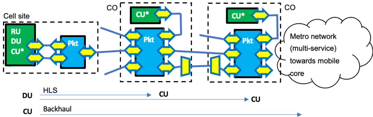
Figure 22: Backhaul and HLS for DRAN and virtual RAN. CU* indicates possible locations for the CU, at the cell site, or at the closest CO. The latter constitutes the VRAN case. The pluggables at the CO sites may be C-temp as indicated by dashed borders for the intraoffice ones.
