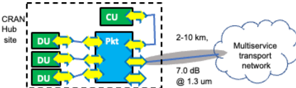
Figure 29: 10 km CRAN backhaul Blueprint (direct P2P, no WDM). The link specified has a gray background. In cases where the CU is located at another location, HLS is illustrated. The pluggables at the CRAN hub site may be C-temp as indicated by dashed borders for the intraoffice ones.
