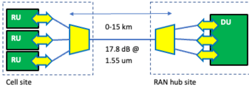
Figure 17: 15 km RU-DU, DWDM passive wavelength multiplexed, P2P or P2MP Blueprint.
