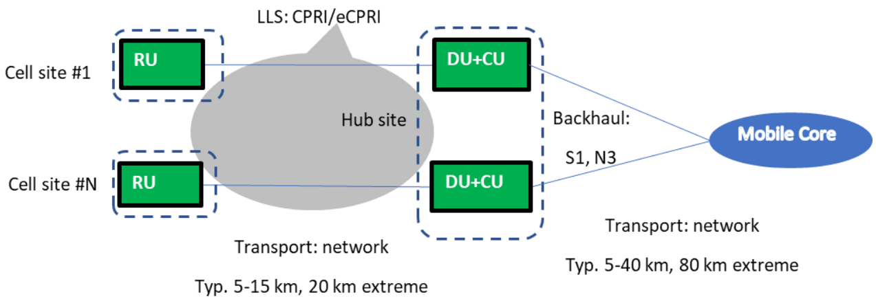
Figure 7: CRAN architecture. The LLS links are highlighted by the gray oval.
