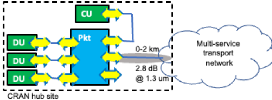
Figure 28: 2 km CRAN hub site intraoffice backhaul direct parallel fiber Blueprint. The link specified has a gray background. In cases where the CU is located at another location, HLS is illustrated. The pluggables at the CRAN hub site may be C-temp as indicated by dashed borders for the intraoffice ones.
