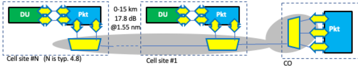
Figure 27: 15 km DRAN backhaul, DWDM passive wavelength multiplexed bus Blueprint. The link specified has a gray background. In cases where the cell site DU is collocated with the CU, backhaul is illustrated. If the CU is located at another location, HLS is illustrated.
