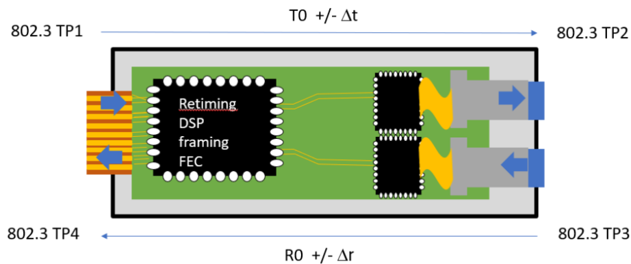
Figure APB.10: measurement points.
