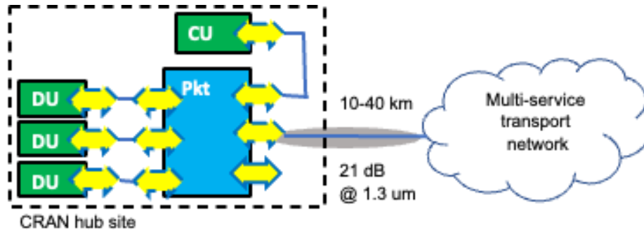
Figure 30: 40 km CRAN hub site backhaul direct parallel fiber Blueprint. The link specified has a gray background. In cases where the CU is located at another location, HLS is illustrated. The pluggables at the CRAN hub site may be C-temp as indicated by dashed borders for the intraoffice ones.
