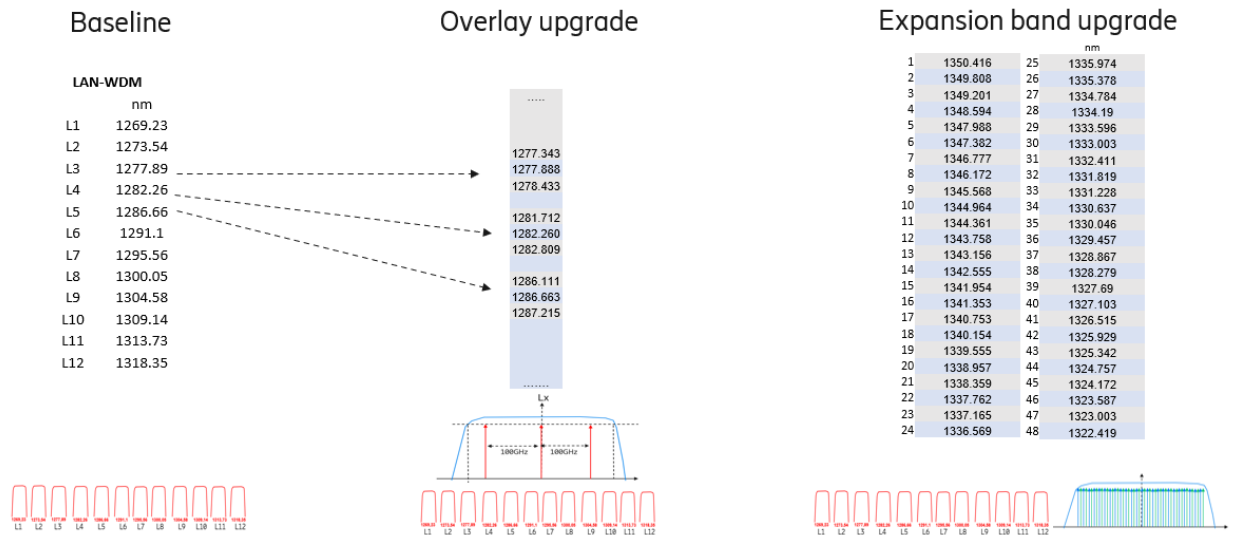
Figure ANA.2: "baseline", "overlay" and "expansion" wavelength grids.
