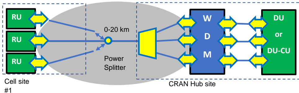
Figure 36: LLS using semi-active DWDM wavelength multiplexed links over a power splitter ODN (WS-WDM-PON).
