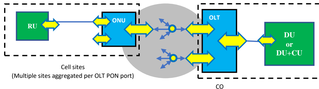
Figure 34: LLS using TDM-PON with separate ONU box.
