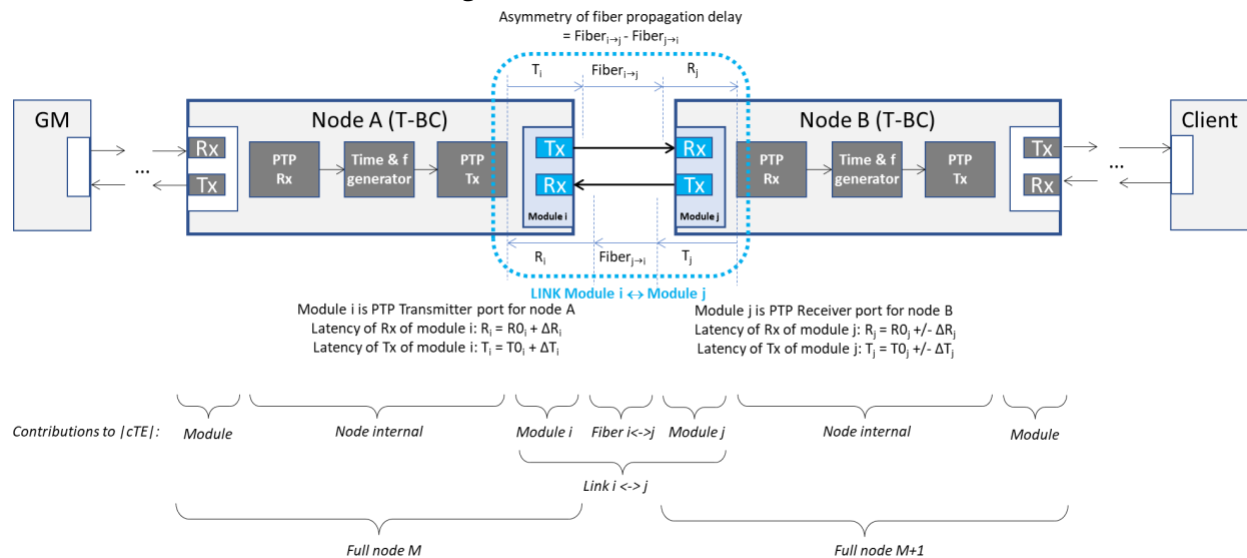
Figure APB.12: Different propagation delay contributions to end-to-end cTE.
